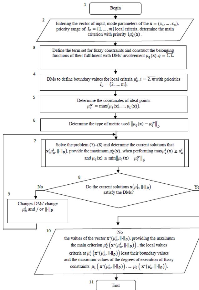
Figure 2. Block diagram of a heuristic method of multicriteria optimization in a fuzzy environment based on a combination and modification of the principles of optimality MC and IP.
